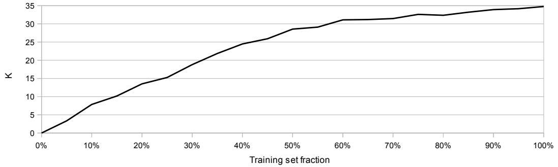
Figure 6.1: K value obtained training the model with different fractions of the original training set
